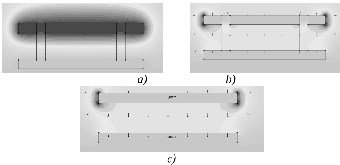
Figure 3 – Distribution of electric potential in the volume of the measuring cell (a), in the volume of the measuring cell without compensating electrodes (b), in the volume of the measuring cell with compensating electrodes (c)
