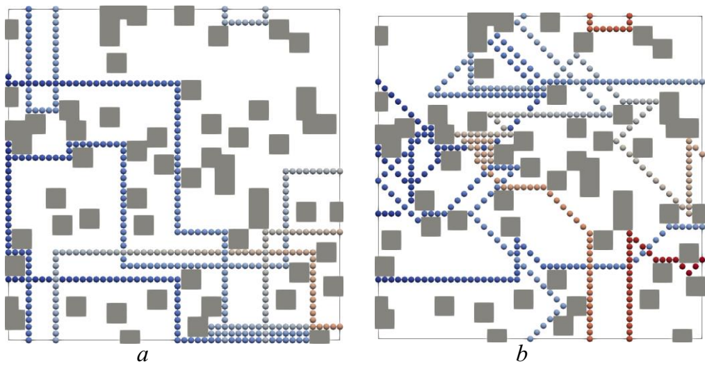
Fig. 3. Random Walk Algorithm: a - model D2Q4, b - model D2Q8
