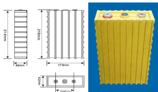
Figure 2 – Lithium-ion battery WB-LYP100AHA
