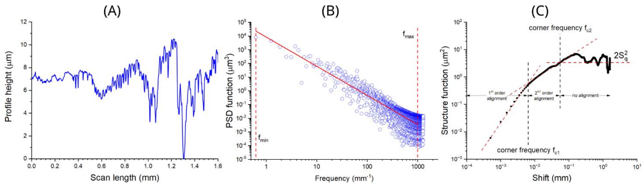
Fig. 1. Example height profile (A), and respective PSD function (B) as well as structure function (C) derived from it
