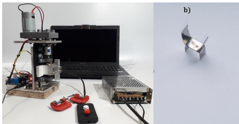
Figure 2 – Breaking force measuring device and exemplary sample (b)
