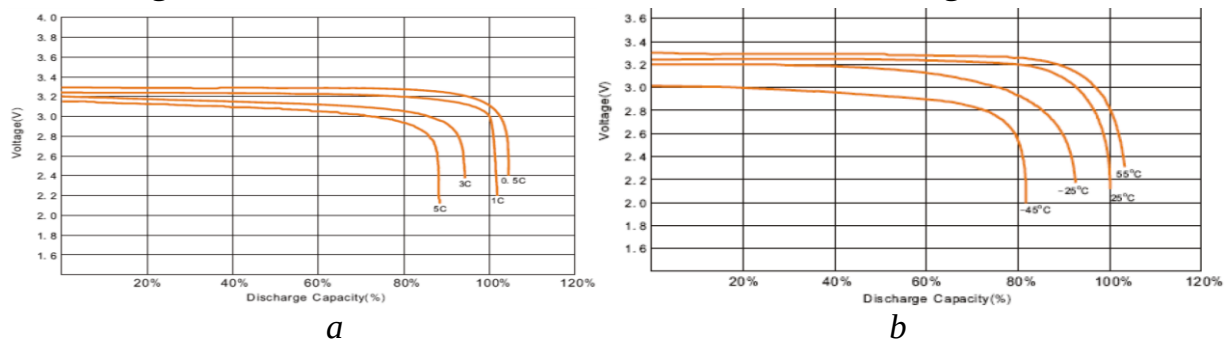
Figure 3 – Discharge characteristics: a – at normal temperature, b – at elevated and lowered temperatures
