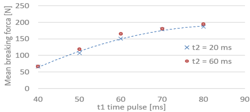
Figure 3 – Mean breaking force values for welds samples
