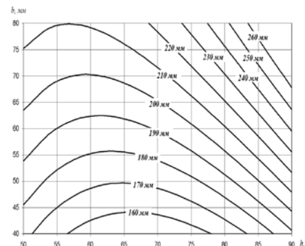
Fig. 3. Additional diagram for size selection of the “wedge”
